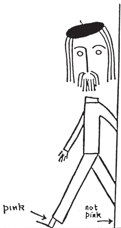
Figure 2. My socks were always of two different colors, as John Bell observed in this cartoon accompanying his paper “Bertlmann’s socks and the nature of reality.” 8,10 The paper, which addressed the difference between quantum and classical correlations, was based on a colloquium, “Conceptual Implications of Quantum Mechanics,” organized by the Hugot Foundation of the Collège de France.
