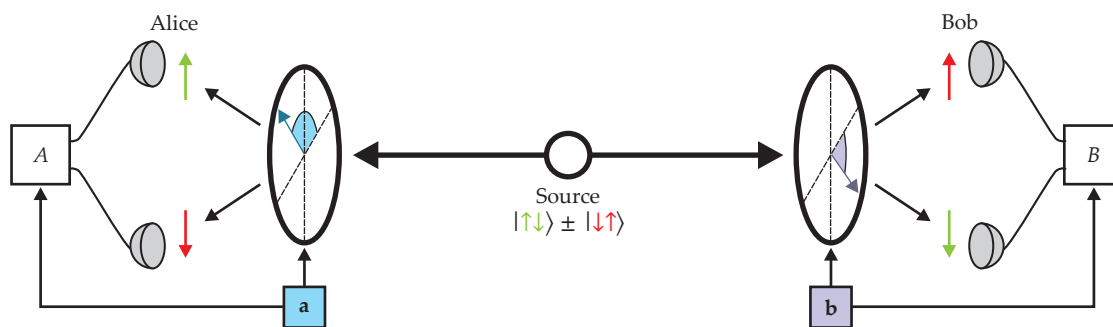
Figure 3. John Bell's famous inequality was derived for the setup illustrated here. A pair of spin- \frac{1}{2} particles are prepared in a state of zero angular momentum, and each propagates freely in opposite directions to the measuring stations called Alice and Bob. Alice measures the spin in a direction a while Bob simultaneously measures in a direction b . In a hidden-variable theory, the measurement results are predetermined; the hidden variables might decree, for example, that if Alice measures her spin up, Bob will measure his down. (Adapted from R. A. Bertlmann, J. Phys. A 47 , 424007, 2014.)
