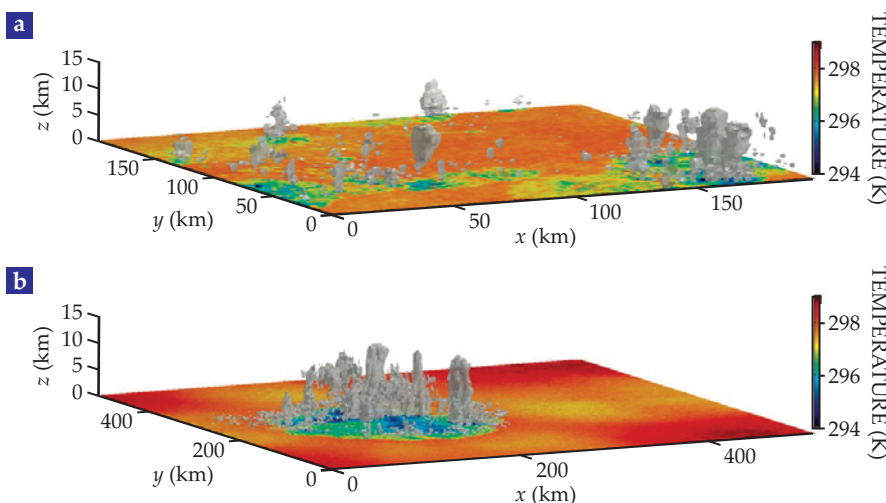
FIGURE 3. IDEALIZED NUMERICAL SIMULATIONS. In the absence of feedback mechanisms, (a) simulated clouds appear disorganized in space. (b) Under the influence of those mechanisms, however, clouds can self-aggregate into a coherent convective structure, and that behavior increases with domain size and temperature. Self-aggregation is associated with a large-scale drying of the atmosphere and enhanced large-scale outgoing radiative cooling to space. Based on observations of relative humidity, researchers have learned that the middle troposphere is consistent with modeled self-aggregation and is on average drier for an atmosphere in which the same amount of precipitation is concentrated into a small number of convective clusters. (Adapted from ref. 1.)
