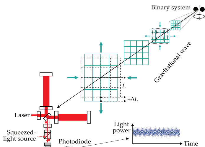
FIGURE 3. GRAVITATIONAL-WAVE DETECTION. A gravitational wave with amplitude \Delta L/L dynamically expands and compresses spacetime perpendicular to its direction of propagation. Laser light propagating along an expanding spacetime axis is redshifted, whereas light moving along a shrinking spacetime axis is blueshifted. The effect is observed with Michelson interferometers that translate those frequency shifts into changes in the power output. All mirrors are suspended as pendulums and are decoupled to the greatest possible extent from environmental forces. The squeezed light reduces photon shot noise at the photodiode such that the sinusoidal signal in the noisy blue data becomes visible. (Adapted from ref. 10.)
