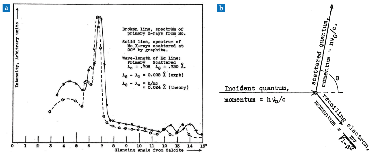
FIGURE 4. TWO DIAGRAM from Compton's 1923 paper in the Physical Review that announced his x-ray scattering results. (a) This plot shows the wavelength-shifted spectrum of molybdenum x rays scattered to an angle \theta of 90 degrees from a graphite block. As the "glancing angle" increases, so does the wavelength that the Bragg spectrometer is sensitive to. (b) This diagram illustrates conservation of momentum and energy for an x ray scattering from an electron. (Reproduced from ref. 2.)
