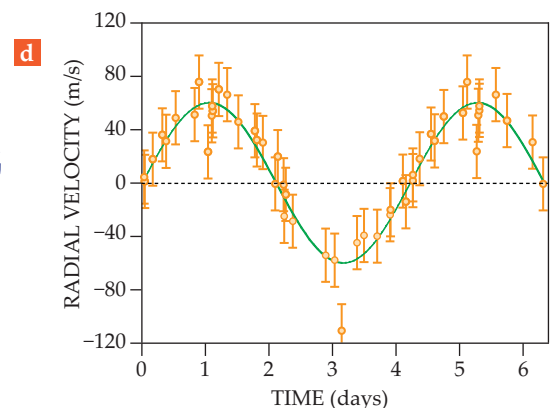
FIGURE 4. THE ORBITAL MOTION of the star 51 Pegasi was detected by the Doppler wobbles of the star and its Jupiter-mass planet relative to the system's center of mass (CM) (a–c). The velocity modulation is 60 m/s (d). (Panels a–c by David Nolte; panel d is adapted from ref. 14.)
