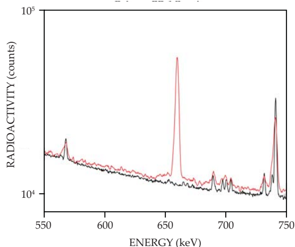
FIGURE 4. IN GAMMA-RAY SPECTROSCOPY , a peak at 662 keV indicates the presence of cesium-137, a ubiquitous fission product of uranium-235. The peak is present in the red spectrum obtained from a piece of the Chicago Pile-1 reactor, which achieved criticality; the piece is part of a collection of the Smithsonian National Museum of American History. However, the peak's noticeable absence in the spectrum obtained from our cube (black) confirms that it was never part of a critical chain reactor.
