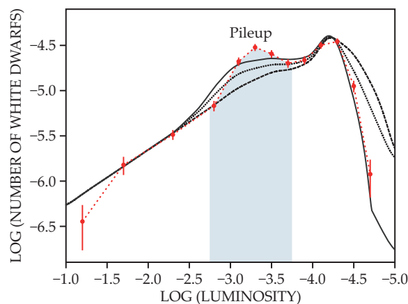
FIGURE 3. THE NUMBER OF WHITE DWARFS (RED DOTS) per unit luminosity per unit volume versus luminosity L/L_{\odot} for stellar masses 0.9\text{--}1.1 M_{\odot} , where L_{\odot} and M_{\odot} are the luminosity and mass of the Sun. The number steadily rises as the luminosity falls until the stars cool to less than 1/1000 of the Sun's luminosity. The plot's peak in the shaded region is a direct observational signature of crystallization. Three model simulations (black lines)
