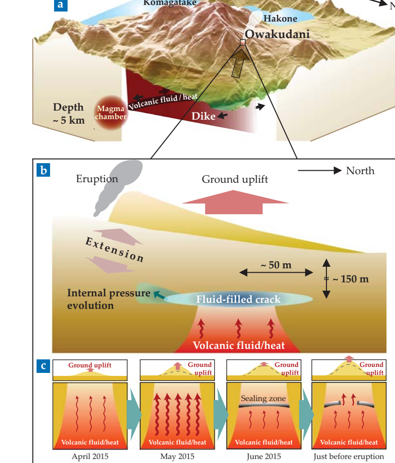
FIGURE 3. SCHEMATIC OF THE PHREATIC ERUPTION PROCESS in the months before Mount Hakone's 2015 eruption. (a) A deep magma chamber beneath nearby Mount Komagatake provides a heat source for the Owakudani geothermal area via a dike that trends north-south. (b) Ground uplift occurs in response to pressure changes in the fluid-filled crack. (c) In the final months before the eruption, heat and fluid influx increases and a crystallized seal allows pressure to build in the fluid-filled crack. Just before eruption, the seal breaks. (Adapted from ref. 1.)
