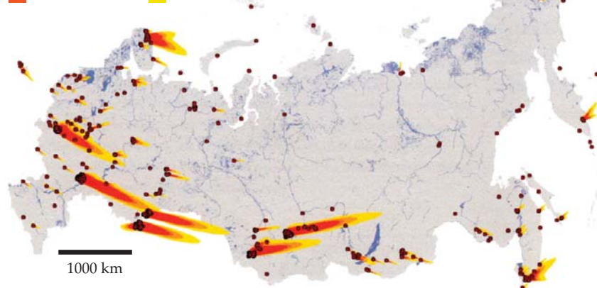
FIGURE 3. FALLOUT PLUMES from a possible US 1289-warhead counterforce attack on Russia's nuclear forces. The largest plumes are from intercontinental-ballistic-missile bases with 30–120 silos each. The largest plumes from the Kola and Kamchatka peninsulas result from attacks on ballistic-missile submarine bases. Smaller plumes throughout the nation are from attacks on mobile missile bases, bomber bases, and nuclear warhead storage facilities. The dots without fallout plumes are from airbursts over nuclear weapons production sites, command headquarters, military radio transmitters, and satellite communications sites; the bursts are assumed to be high enough that their fireballs would not contact the ground and produce local fallout. (Adapted from ref. 7.)
