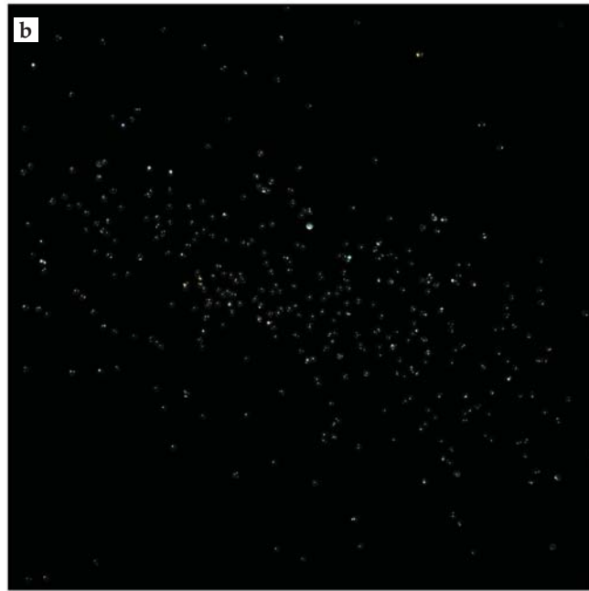
FIGURE 4. A HIDDEN, TINY GALAXY. Reticulum II (Ret II) is an ultrafaint dwarf galaxy on the outskirts of the Milky Way. (a) This image shows all the stars in the direction of Ret II. The horizontal bars on the brighter stars arise from saturation effects. (b) Sophisticated image search algorithms can identify the stars in panel a that are members of Ret II. A coherent structure is clearly visible. (Courtesy of the Dark Energy Survey/Fermilab.)
