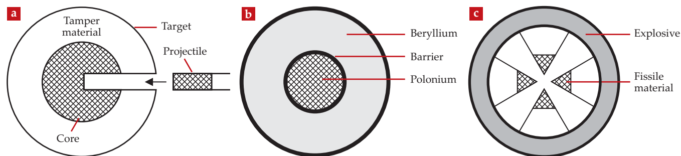
FIGURE 3. CONCEPTS FOR TRIGGERING an atomic bomb. (a) In the shooting method, a projectile of fissile material is propelled into the target. Neither piece alone constitutes a critical mass by itself, but when combined, they do. (b) The initiator, the device that starts the chain reaction, contains a few milligrams of polonium surrounded by a layer of beryllium. When the barrier is ruptured by the assembling bomb core, the elements mix, and the alpha- n effect creates a torrent of neutrons to initiate the reaction. (c) In the implosion method, wedge-shaped pieces are pushed together to form a critical mass by detonating an explosive. Implosion is faster than the shooting method and is more suitable for plutonium-based weapons.
