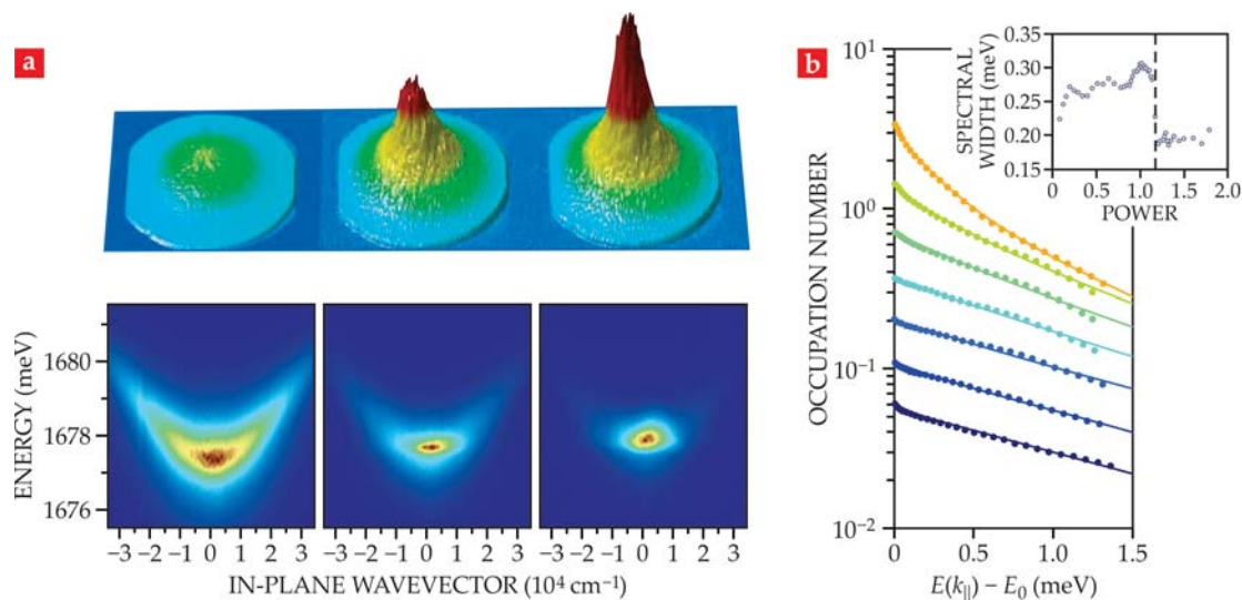
FIGURE 3. THE BOSE-EINSTEIN CONDENSATION OF POLARITONS carries clear, experimentally observable hallmarks. (a) As polariton density increases (left to right) above the condensation threshold, the polaritons' in-plane momenta, evidenced by the angular distribution of their light emission, peaks sharply at zero (top), and their energies and momenta converge on the minimum of the dispersion curve (bottom). That curve shifts slightly upward due to interaction effects as the polariton density increases. Here, regions of parameter space colored red correspond to those that produced the highest density of photon counts. (Adapted from ref. 5.) (b) In experiments that achieve full equilibrium, the evolution of the observed energy distribution (dots), plotted as a function of wave number k_{\parallel} , is well described by the Bose-Einstein distribution (curves). Here, polariton density increases as curves change from purple to orange, with the orange curve corresponding to a system on the verge of condensation. The inset shows the sharp decrease in the spectral width of the polariton emission line as pump power crosses the threshold for condensation, indicated by the dashed line. (Adapted from ref. 7.)
