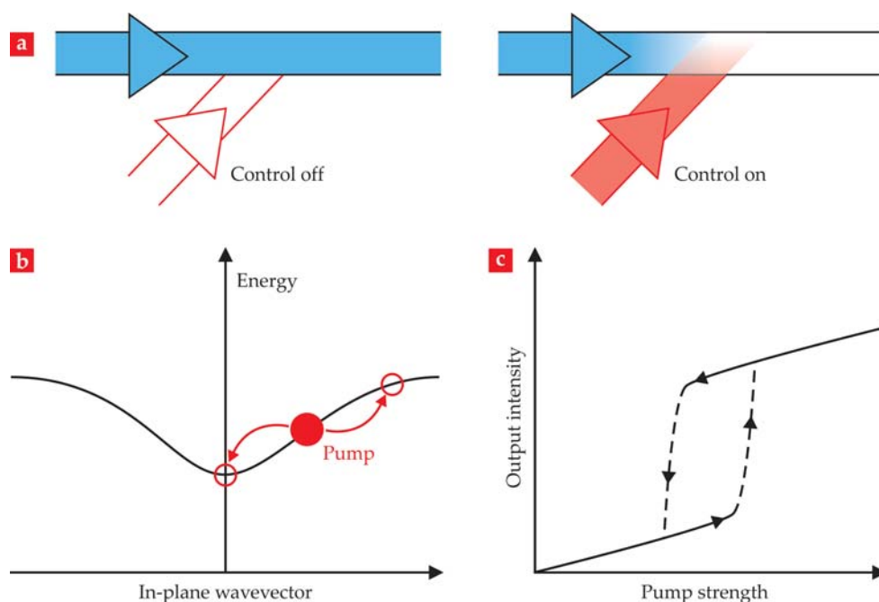
FIGURE 4. OPTICAL SWITCHES
