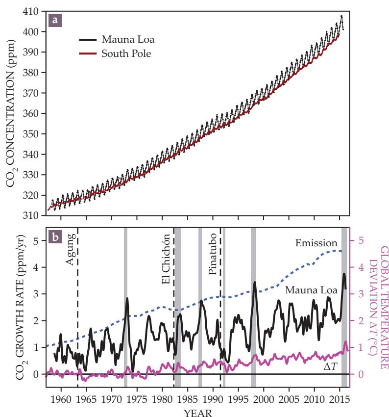
FIGURE 1. THE RELENTLESS CLIMB of atmospheric carbon dioxide. (a) Since the late 1950s, atmospheric \text{CO}_2 concentrations have been measured at the Mauna Loa Observatory in Hawaii and the South Pole Observatory in Antarctica. The prominent annual cycles in the Mauna Loa record reflect the seasonal uptake and release of \text{CO}_2 by plants and soils in the Northern Hemisphere. The difference in \text{CO}_2 between Mauna Loa and the South Pole has grown larger as fossil-fuel emissions have increased because emissions are concentrated in the Northern Hemisphere. (b) The annual growth rate of \text{CO}_2 at Mauna Loa and the \text{CO}_2 growth rate expected from fossil-fuel emissions are plotted with the deviation in global temperature \Delta T relative to the 1950–80 average. Except during strong El Niño conditions in 1972–73 and 1997–98, the observed \text{CO}_2 growth rate is lower than expected from fossil-fuel emissions because of \text{CO}_2 uptake by the ocean and by plants and soils on land (see box 1). When temperatures are warm, as commonly found during El Niño periods (gray shading), \text{CO}_2 increases more rapidly. Strong volcanic eruptions (dashed vertical lines) generally result in cooler temperatures and slower rates of change in \text{CO}_2 . (Atmospheric \text{CO}_2 concentration data courtesy of Scripps Institution of Oceanography, global temperature data courtesy of NASA, and fossil-fuel emissions data courtesy of Oak Ridge National Laboratory. Emissions estimates for 2014–15 from ref. 16.)
