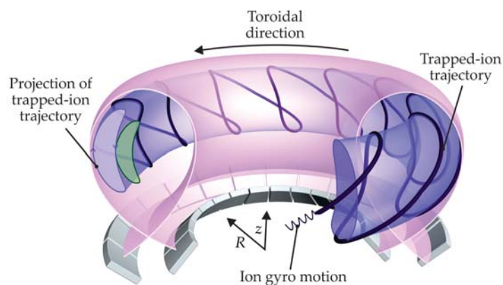
Figure 1. A tokamak is a bagel-shaped vessel that confines a hot plasma (bounded by the pink shell) within a magnetic field that twists around the torus in a gentle helix. The field arises from a combination of external magnets (not shown) and guides electrically charged particles into so-called passing and trapped-ion orbits. In the case of the latter, because the magnitude of the net applied field falls off with radius R from the axis of the torus, a trapped ion follows a banana-shaped trajectory (black, in the purple shell). While tracing that path, the ion also experiences small-scale oscillations, or gyro motion, about the magnetic field. Projections of two ion trajectories (purple and green) are shown at left. The silver rails below the plasma collect helium ash and other debris from the fusion reaction. (Courtesy of EUROfusion.)
