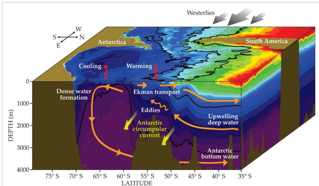
Figure 1. Dynamics in the Southern Ocean. The westerly winds combine with the Coriolis force to drive a northward flow, known as the Ekman transport, at the ocean's surface. The Ekman transport shifts the light surface waters northward, thereby tilting the density contours—shown as colors ranging from red (surface light water) through blue (deep dense water)—up from the horizontal. The latitudinal variation in the westerlies creates a divergence in the Ekman transport, which causes water to upwell along the sloping density layers from the deep ocean to the surface. (Eddies and the flow of the strong eastward Antarctic circumpolar current over topographic ridges also influence the upwelling, as outlined in box 2.) Upon reaching the upper ocean, the upwelled waters split into two pathways: Water that reaches the surface close to Antarctica's sea ice is cooled, sinks along the continental shelf, and is transformed into dense bottom water; water that surfaces north of the sea-ice edge is warmed and flows northward with the Ekman layer. 4
