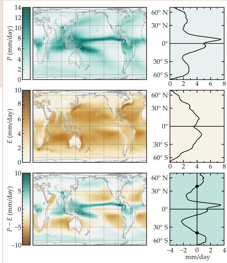
Figure 3. Average precipitation ( P ), evaporation ( E ), and the difference between them are mapped on the left for the years 1981–2010. The values are replotted as latitude averages on the right. Subtropical deserts and tropical rainforests are sustained by water deficit and water surplus, respectively. Edges of the tropical belt can be located where precipitation and evaporation balance each other (diamonds in lower right plot).
