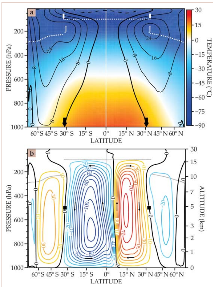
Figure 4. The tropical belt's edges can be located from the distributions of atmospheric temperature and winds. (a) In this plot of data averaged over 30 years (1981–2010), a dome of warm air at the equator cools with increasing latitude and decreasing atmospheric pressure (or equivalently, increasing altitude). Black lines mark contours of constant eastward wind speed in units of meters per second. Inside much of the dome, the winds flow westward. At the zero contour, they calm and, with increasing latitude or altitude, reverse direction. The tropopause, the boundary between the troposphere and the stratosphere, is marked by the white dotted line. The edges of the tropical belt may variously be defined as being at the jet-stream cores marked “J,” at the transition from westward to eastward surface winds marked by black arrows, or where the tropopause abruptly changes altitude (white arrows). (b) The mass stream function plotted here measures the rate of mass transport along meridians between a given altitude and the top of Earth's atmosphere as a function of latitude. Contours of equal mass transport are in units of 10^9 kg/s, with clockwise circulation shown in red and counterclockwise circulation in blue; black lines mark transitions between the circulation patterns. Black squares mark the edges of the subtropical stream function at 500 hPa, halfway through the vertical extent of the Hadley cell.
