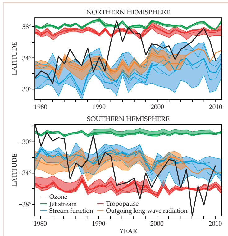
Figure 5. Changes in the edge locations of the Northern and Southern Hemispheres, 1979–2012. The plots include five annually averaged metrics that independently measure the edges of the tropical belt. They are based on reanalyses (see the box on page 41) of the tropopause (red), stream function (blue; see figure 4), and jet stream (green), and on satellite measurements of ozone (black) and thermal IR radiation (orange). Where multiple estimates of a particular metric are available, they are shown as light solid lines, surrounded by shading that indicates their range; a heavy line indicates their median. (Adapted from figure 2.40 of ref. 7.)
