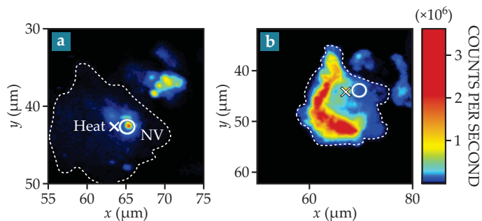
Figure 5. Nanoscale thermometry senses the living and the dead.
