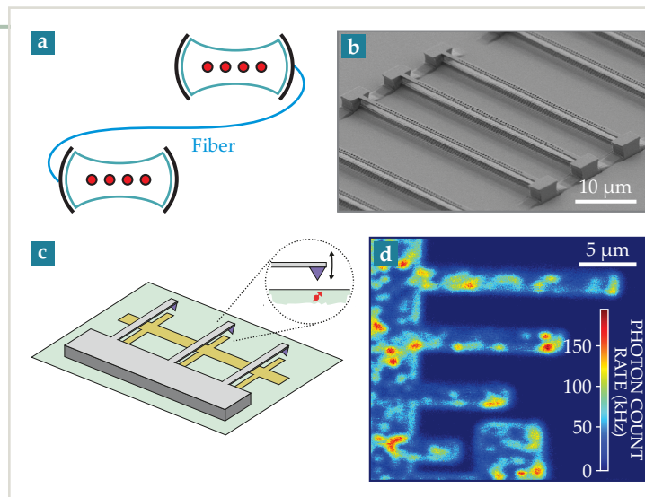
Figure 3. Quantum interfaces for atom-like systems.
