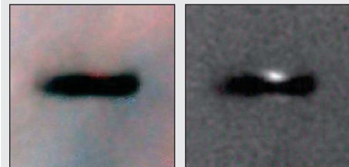
Figure 1. A protostellar disk in the Orion Nebula, viewed edge-on by the Hubble Space Telescope . The left image was generated with a camera that is sensitive to radiative emission lines from the gaseous disk; the right image was taken with a filter that blocks those lines. With the disk gas less prominent, reflected light from the central star is clearly visible. (Courtesy of Mark McCaughrean, C. Robert O'Dell, and NASA.)
