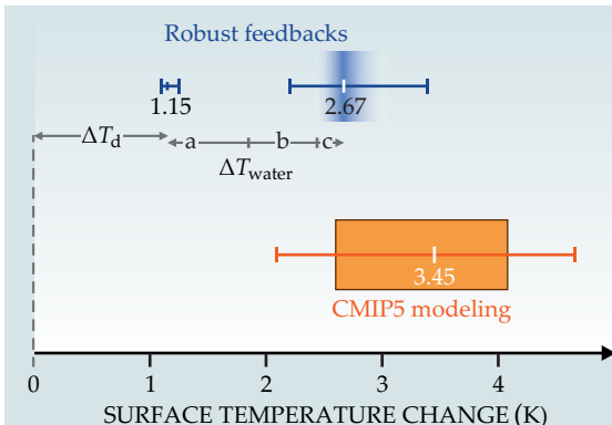
Figure 4. How much does the temperature of Earth's surface change from doubling the carbon dioxide in the atmosphere? Comprehensive climate models from the coupled-model intercomparison project (CMIP5) yield a median estimate of 3.45 K bounded in the orange box by the 25%–75% spread over the total range of values. Shown in blue are the estimates of the temperature change based on well-understood feedback processes. In the absence of the effects of water, one expects a warming \Delta T_d of about 1 K. Water in the atmosphere increases that dry response by an additional 1.5 K. The amplification includes contributions from processes described in the text: the combined water-vapor and lapse-rate feedbacks (a), the cloud-greenhouse feedback (b), and the surface-albedo feedback (c).
