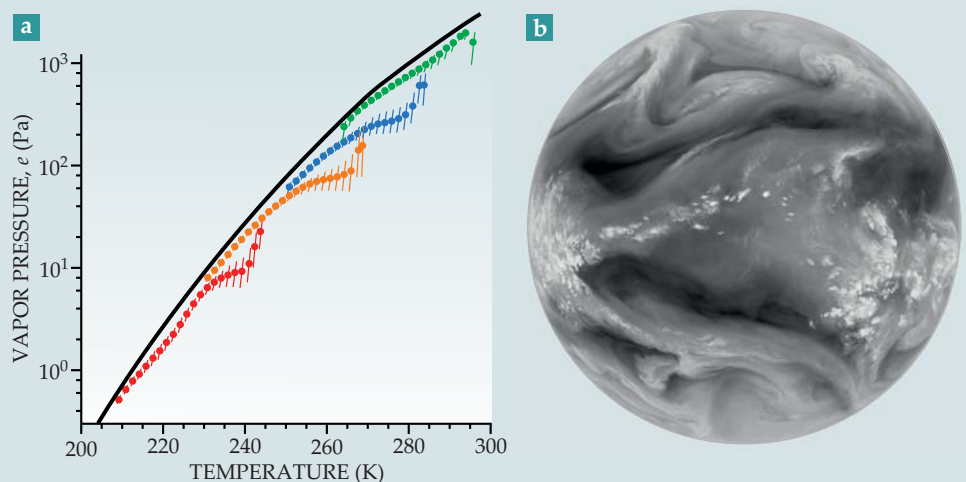
Figure 2. The atmospheric vapor pressure as a function of temperature (a) is bounded by the atmosphere's vapor pressure when saturated with water (solid line). The data are shown as the median (dot) and range (error bar) of 228 monthly values at different isobaric levels—900 hPa (green), 700 hPa (blue), 500 hPa (orange), and 300 hPa (red). (Data are provided by the European Centre for Medium-Range Weather Forecasts.) (b) Based on satellite measurements of radiation emitted at 6.2 \mu\text{m} , this map reveals the relative humidity of the middle and upper troposphere. It also reveals how closely humidity levels are tied to atmospheric circulation patterns: Pronounced dry regions (dark) show large-scale descending motions of air concentrated in the subtropics. Clouds, regions of complete saturation, are visible as white features. (Image from Meteosat.)
