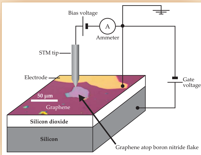
Figure 1. A scanning tunneling microscopy (STM) setup used to measure graphene’s local density of states. The monolayer graphene sample (purple) is deposited atop flakes of boron nitride to improve the uniformity of the background charge distribution. From variations in the measured current as a function of bias voltage, one can infer the sample’s local density of states. When the graphene is configured atop silicon dioxide and silicon sublayers, its charge-carrier doping can be manipulated with a gate voltage. (Adapted from ref. 3.)
