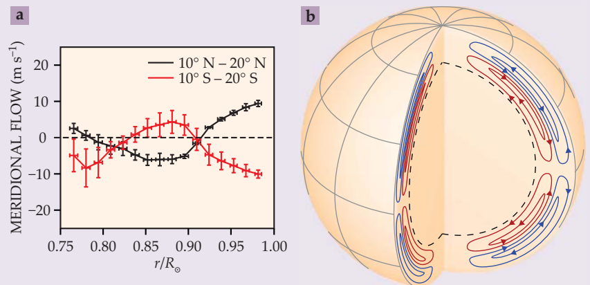
Figure 2. Profiling the depths. (a) Time-distance helioseismology measurements of subsurface velocity profiles in the Sun's northern (black) and southern (red) hemispheres suggest that the meridional flow of plasma is poleward at radial distances r greater than about 0.9 R_{\odot} , equatorward between roughly 0.8 R_{\odot} and 0.9 R_{\odot} , and poleward below that ( R_{\odot} is the solar radius). By convention, northerly flow is positive. (b) The observed profiles suggest that two distinct circulation cells transport solar plasma from the equator to the poles and back. The black dashed line indicates the bottom of the convective zone. (Adapted from ref. 2.)
