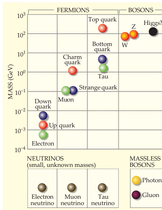
Figure 1. Fundamental particles of the standard model and their approximate masses. Three generations of fermions form the building blocks for matter; forces are carried by the fundamental bosons. Except for the newly discovered particle, all the fundamental bosons have spin 1; the putative Higgs is the first observed fundamental particle with spin 0.
