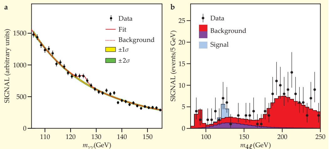
Figure 3. (a) The two-photon ( \gamma\gamma ) mode as observed by the CMS team. The dotted red line is the expected background from non-Higgs processes, and the thin yellow and green stripes are the expected uncertainties of the background predictions. The bump at 125 GeV is attributed to Higgs decays. (Adapted from ref. 2.) (b) The ATLAS team's data for the four-lepton ( 4\ell ) mode. The peak attributed to the Higgs, again at 125 GeV, is shaded in light blue. (Adapted from ref. 3.)
