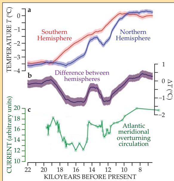
Figure 2. The world-wide array of paleothermometers makes possible (a) separate mean-temperature chronologies for the Northern and Southern Hemispheres. (b) The difference (north minus south) between the measured hemispheric temperatures. (c) The variation of the Atlantic meridional overturning circulation, a northward surface current that perennially transfers heat from the South Atlantic to the North Atlantic. (Adapted from ref. 1.)
