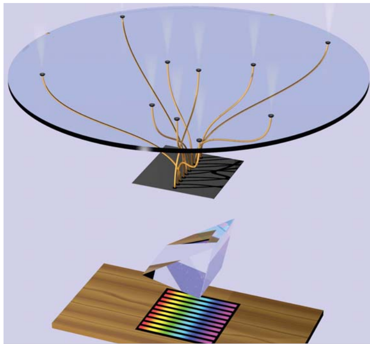
Figure 1. Spectra of many stars or galaxies can be obtained simultaneously in a single field of view by aligning the entrance apertures of optical fibers with the images of individual sources in a telescope's focal plane. The fibers' downstream ends line up along an aperture in a mask that defines the entrance slit for the spectrographic grating (represented here by a prism) that creates separate parallel spectra for the different sources. (Courtesy of A. McGrath.)
