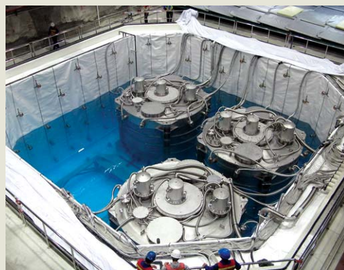
Figure 1. Three electron antineutrino detectors in the far hall of the Daya Bay experiment sit in a water-Cherenkov bath that unmasks cosmic-ray interlopers. The hall, several hundred meters underground, is about 2 km from an array of six power reactors. Each detector measures the \bar{\nu}_e flux from the reactors by recording light flashes due to \bar{\nu}_e collisions in its 20 tons of liquid scintillator.
