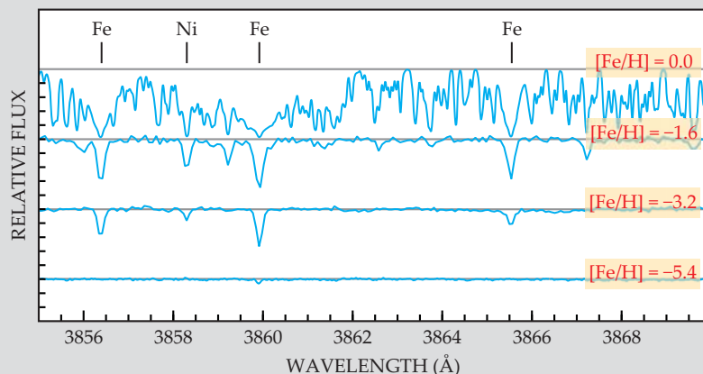
Figure 4. HE 1327–2326, the most iron-poor star yet discovered (as measured by the logarithmic abundance ratio [\text{Fe}/\text{H}] ), has just a tiny absorption-line bump visible in the lowest of the four absorption spectra shown here. The stars generating the other three spectra are, from top to bottom, the Sun, G66–30, and G64–12. Evidently, the variations in line strength reflect the decrease in stellar metallicities. Four neutral elemental absorption lines are indicated near the top of the plot. (Adapted from ref. 18.)
