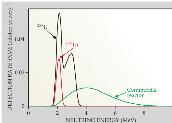
Figure 3. Expected detection rates from various sources of electron antineutrinos ( \bar{\nu}_e ) per kiloton of scintillator liquid for a scintillation detector at a typical continental site, plotted against the \bar{\nu}_e 's incident energy. The 1.8-MeV cutoff is the threshold for the inverse-beta-decay reaction that reveals the \bar{\nu}_e . Below 3.5 MeV, the expected spectrum is dominated by beta-decay \bar{\nu}_e s from the decay chains of uranium-238 and thorium-232 in Earth's crust and mantle. The spectrum of \bar{\nu}_e s from nuclear reactors peaks near 4 MeV, where the geoneutrino spectrum has already petered out, making it possible to distinguish between natural and reactor sources.
