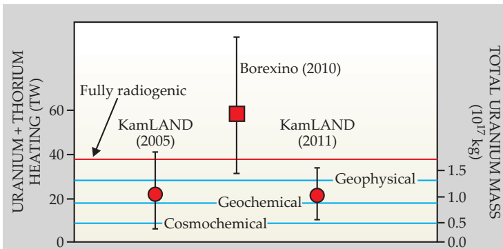
Figure 4. Heating of Earth by uranium and thorium decay, as deduced from three geoneutrino experiments. 3–5 Both KamLAND measurements are consistent with the predictions of the principal classes of Earth models (blue lines). But the 2011 measurement excludes, with 97% confidence, the fully radiogenic model (red) that assumes no remaining primordial heat. The right-hand axis translates the U + Th heating power into the deduced total mass of U in the mantle and crust.
