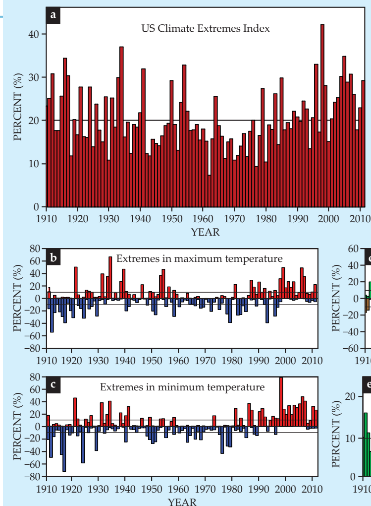
Figure 2. Weather and climate extremes.
