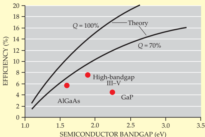
Figure 3. Some recent efficiency measurements for tritium betavoltaics using aluminum gallium arsenide, 5 gallium phosphide, 7 and a high-bandgap III–V semiconductor, 11 compared with the theoretical maximum efficiency as a function of bandgap. Theoretical curves are shown for collection efficiencies Q (the current generated relative to the maximum possible current) of 100% and 70%.
