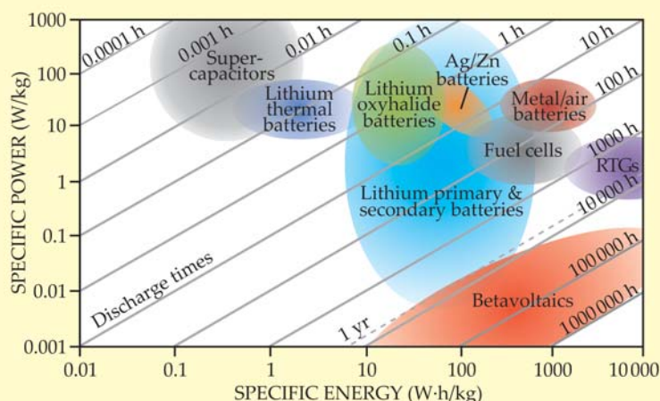
Figure 4. Betavoltaics supply low power over a long lifetime, making them unique among energy-storage devices, including chemical batteries, fuel cells, supercapacitors, and radioisotope thermoelectric generators. RTGs use more aggressive radioisotopes, such as polonium-210 or plutonium-238, to generate heat, which is then converted into electricity via the Seebeck effect. (For more on chemical batteries and supercapacitors, see the article by Héctor Abruña, Yasuyuki Kiya, and Jay Henderson in PHYSICS TODAY , December 2008, page 43.)
