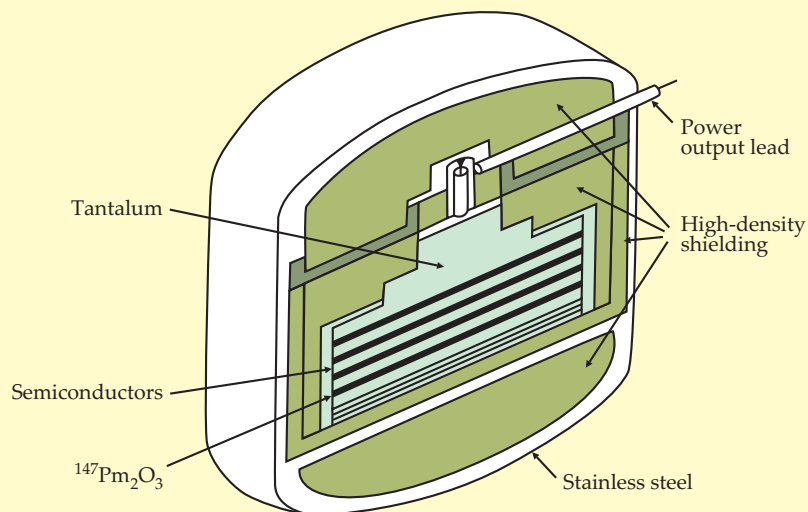
Figure 1. The Betacel model 400 , an early betavoltaic battery powered by promethium-147. The device was produced for use in cardiac pacemakers.
