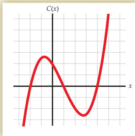
Figure 2. Friedmann's fundamental cubic C(x) , given by equation 4 in the text, is plotted here against cosmic radius x for arbitrary values of the free cosmological parameters \lambda and A . Their true values determine whether C(x) has 0 or 2 positive roots, and they define three general scenarios of cosmic evolution. One gets additional limiting-case scenarios if the two positive roots are degenerate. Changing the sign of the linear term in C(x) to describe a cosmos with negative curvature yields still more scenarios.
