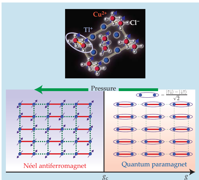
Figure 2. Thallium copper chloride ( \text{TlCuCl}_3 ) exemplifies another quantum phase transition. 2 The \text{Cu}^{2+} ions boast active spin- \frac{1}{2} states. At ambient pressure, the spins pair into dimers and form singlet bonds (|\uparrow\downarrow\rangle - |\downarrow\uparrow\rangle)/\sqrt{2} , as indicated by the ellipsis (top). The behavior is similar to that of a so-called dimer antiferromagnet on a square lattice. The solid red lines represent strong spin interaction with a positive exchange coupling J > 0 , while the dashed green lines have a weaker exchange coupling J/g , with g \geq 1 . The ground state of \text{TlCuCl}_3 is similar to the dimerized, large- g ground state of the dimer antiferromagnet, which behaves like a quantum paramagnet (right). For \text{TlCuCl}_3 , g is inverse pressure. As the pressure increases and g decreases, \text{TlCuCl}_3 undergoes a quantum phase transition to Néel antiferromagnetic order, in which neighboring spins are antiparallel. In the dimer antiferromagnet model, the transition to Néel order occurs at a quantum critical point g = g_c .
