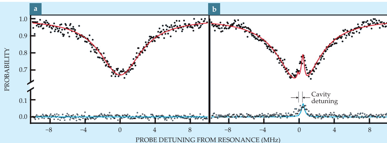
Figure 2. The probabilities of transmission through the cavity (red) and of emission into it (blue) are measured by the two photon-counting detectors sketched in figure 1. (a) The spectrum shows a drop in transmission as the probe laser frequency is swept through the resonance frequency of one of the two atomic transitions ( |f\rangle \rightarrow |e\rangle ) in figure 1). When the cavity mode doesn't match the other atomic transition frequency, the probe photons behave as if the mirrors are not there and no photon field builds up between them. (b) When the cavity mode is close to the other transition frequency ( |g\rangle \rightarrow |e\rangle ), the vacuum-induced transparency spectrum shows the telltale increase in light transmission in a narrow frequency window. (Adapted from ref. 2.)
