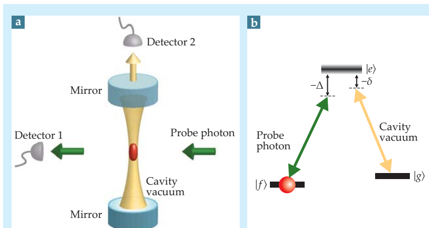
Figure 1. Vacuum-induced transparency. (a) Photons in a probe pulse experience Raman scattering as they interact with a cloud of three-level cesium atoms (red) in an optical cavity. The photons are absorbed and quickly emitted into the cavity, where, after some time delay they are reabsorbed and reemitted collectively—that is, in a way mediated by the response of all the atoms—as an identical probe pulse. Detectors 1 and 2 measure the probe transmission and scattering in the cavity, respectively. (b) During the interaction, two transitions from Cs hyperfine states |f\rangle and |g\rangle to an excited state |e\rangle are simultaneously driven by the probe field and the cavity field, respectively. When both fields are either on resonance or detuned from it by the same amount, \delta \approx \Delta , coherence between the two hyperfine states cancel the absorption. (Adapted from ref. 2.)
