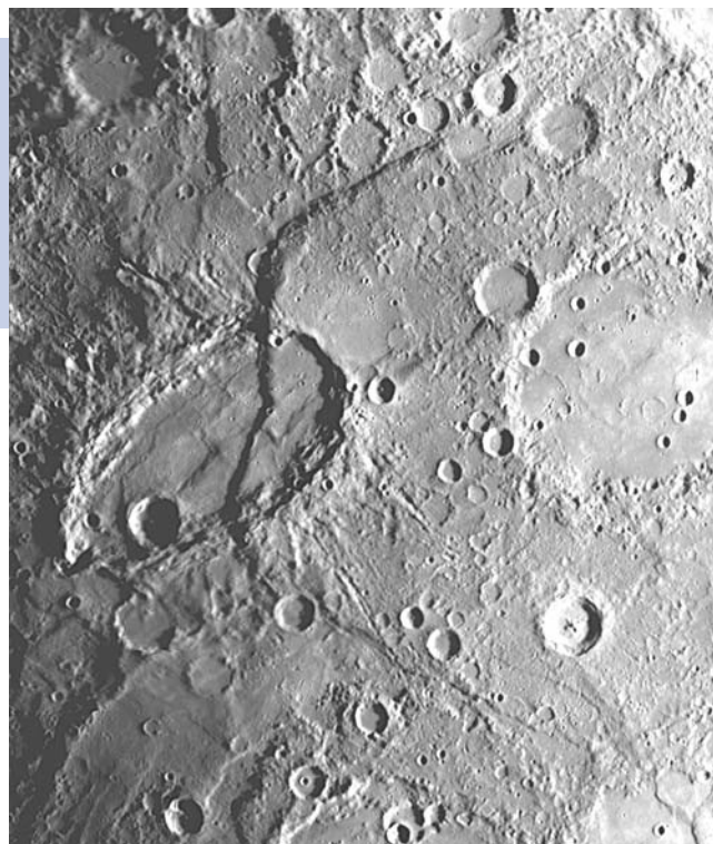
Figure 3. Beagle Rupes , a prominent scarp imaged during MESSENGER 's first Mercury flyby on 14 January 2008, is more than 600 km long and offsets the floor and walls of the elliptically shaped (220 km by 120 km) impact crater Sveinsdóttir, named for the Icelandic painter and textile artist. Beagle Rupes, named for the British naval vessel on which Charles Darwin sailed, is one of the most arcuate of the scarps seen on Mercury to date. 9 (Courtesy of NASA/Johns Hopkins University Applied Physics Laboratory/Carnegie Institution of Washington.)
