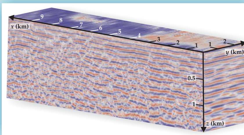
Figure 5. A three-dimensional reflection image of the geology beneath the Libyan desert, based on data obtained by cross-correlating 11 hours of ambient noise. The horizontal stripes indicate discontinuities in Earth's crust due to the juxtaposition of different rock types. Such images are essential for the exploration and production of oil and gas. (Adapted from ref. 15.)
