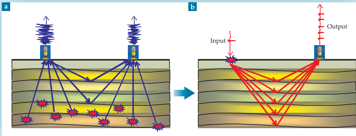
Figure 4. Retrieving the reflection response from ambient noise. (a) Consider an arbitrary, inhomogeneous, lossless medium with noise sources (red) buried in its subsurface and two geophones at its free surface. Those noise sources send waves that reach the geophones directly or after reflecting from subsurface discontinuities. (b) The cross-correlation of noise signals recorded by the two geophones reveals the same reflection response that would be observed by one of the geophones if there were an impulsive source at the position of the other.
