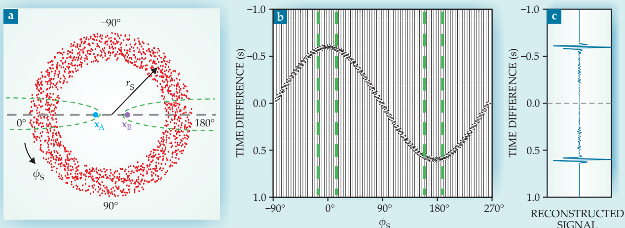
Figure 2. Green function retrieval in a two-dimensional open system. (a) Point sources of noise (red dots) whose positions are denoted by radius r_s and azimuth \phi_s send waves to receivers at \mathbf{x}_A and \mathbf{x}_B . The dashed lines delimit zones in which the cross-correlation of noise recorded at receivers A and B does not, to first order, depend on the angle \phi_s . (b) The cross-correlation of signals that arrive at A and B from each source is plotted as a function of the lag time of the cross-correlation and source azimuth \phi_s . The dashed lines delimit zones where waves constructively interfere. (c) The sum of the correlations in the plot yields two waves at \pm 0.6 s that propagate between the receivers in opposite directions and are described by the Green function and its time-reversed counterpart G(\mathbf{x}_A, \mathbf{x}_B, t) + G(\mathbf{x}_A, \mathbf{x}_B, -t) . (Adapted from K. Wapenaar, J. Fokkema, R. Snieder, J. Acoust. Soc. Am. 118 , 2783, 2005.)
