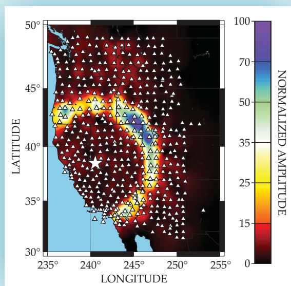
Figure 3. A large array of seismometers (white triangles) in the western US captures the seismic response of a virtual source (white star), located just southeast of Lake Tahoe, California, at a moment in time. The snapshot, taken 200 s after a virtual impulse, was obtained by cross-correlating three years of ocean-generated ambient noise recorded at the station denoted by the star with noise recorded at each of the other stations. The result is a surface wave that propagates from the virtual source outward through the other stations in the array. The approach offers an unprecedented illumination of Earth's crust. (Adapted from ref. 12.)
