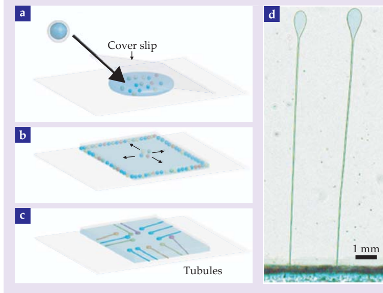
Figure 5. Coaxed by confinement, lipid vesicles assemble into tubules. (a) The lipid vesicle solution is first confined to the thin film between a glass plate and a square cover slip. (b) In a process similar to coffee-ring formation, evaporation of the confined liquid causes an outward capillary flow, which carries the vesicles toward the edge of the cover slip. (c) There, the vesicles organize into inward-protruding tubules of up to 1 cm or more in length, each capped by a compartmentalized head. (d) A microscopy image shows lipid tubules entrapping a blue aqueous dye. (Adapted from ref. 16.)
