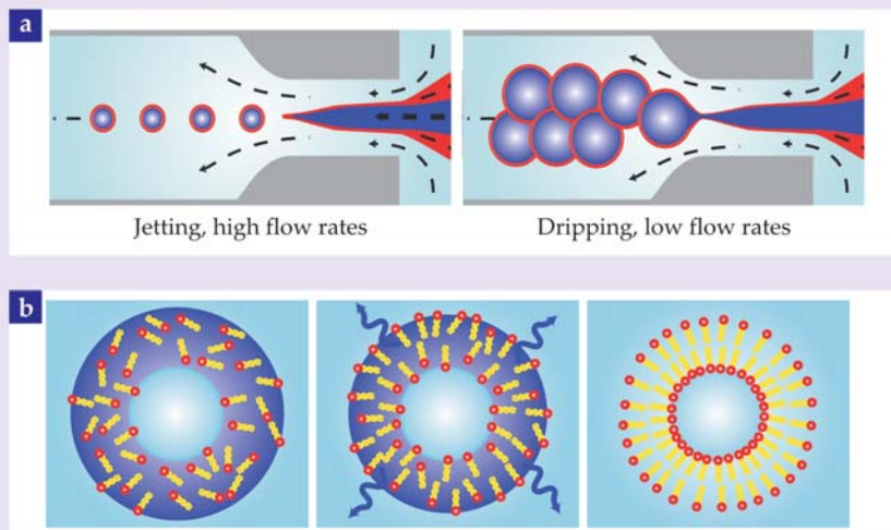
Figure 3. Double emulsions , liquids that contain “bubbles within bubbles,” provide a versatile medium for self-assembly. (a) A double emulsion can be produced by the coordinated flow of three fluids in a microfluidic device. A high flow rate of the inner fluid (dark blue) combined with a low flow rate of the middle fluid (red) leads to jetting; low flow rates for both the inner and middle fluids result in dripping. The outer, continuous fluid phase is shown in light blue. (b) Vesicles can be made by dissolving surfactants in the oil phase of a water-oil-water double emulsion. When the oil is evaporated, it leaves behind the vesicle, a self-assembled, spherical bilayer of surfactants that encapsulates an inner water droplet. If diblock copolymer is used instead of surfactant, the structure is known as a polymersome.
