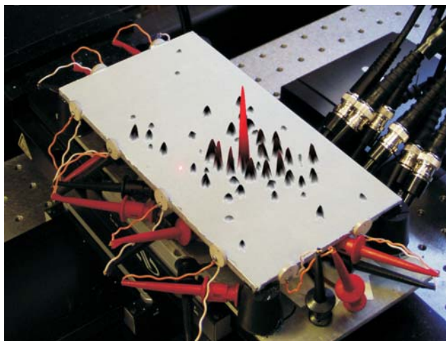
Figure 2. Time reversal in the lab. A source on the underside of a thin aluminum plate, near its center, emits a 20- \mu s strain pulse. The resulting displacements arriving at the plate's edges are recorded by eight detectors arrayed along the perimeter. The recorded signals are time-reversed and rebroadcast from the detectors. A laser vibrometer scans the plate's surface and maps the vertical component of its velocity due to vibrations created by the rebroadcast. The superposed peaks display the velocity map at the moment when the rebroadcast signals focus to reveal the original source (red peak). The lesser peaks are due to reflections and other secondary sources. (Adapted from ref. 6.)
