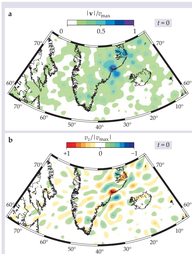
Figure 5. For a glacial earthquake in Greenland, vertical-displacement signals recorded at 146 seismic stations worldwide were frequency-filtered, time-reversed, and rebroadcast into a model Earth to produce these surface-velocity fields for southern Greenland at the moment of focus, which in the time-inverted record corresponds to the instant of the quake's onset. (a) The absolute-velocity field |v| indicates two sources near opposite ends of a glacier on Greenland's east coast. (b) The v_z field, which maps the vertical component of surface velocity at the quake's onset, reveals that the eastern source, near the glacier's front, was thrusting down while the western source, near its upstream end, was thrusting upward. (Adapted from ref. 12.)
