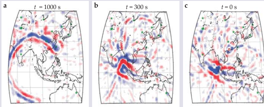
Figure 4. The great Sumatra earthquake of 2004. The quake, lasting about 400 s, resulted from a 1200-km-long rupture between tectonic plates. Seismic records from 165 stations worldwide were time-reversed and rebroadcast into a model Earth. The three maps, each extending from Siberia to Australia, show the propagation of the vertical displacement field thus deduced in reverse time order, labeled by time t since the quake's onset.
