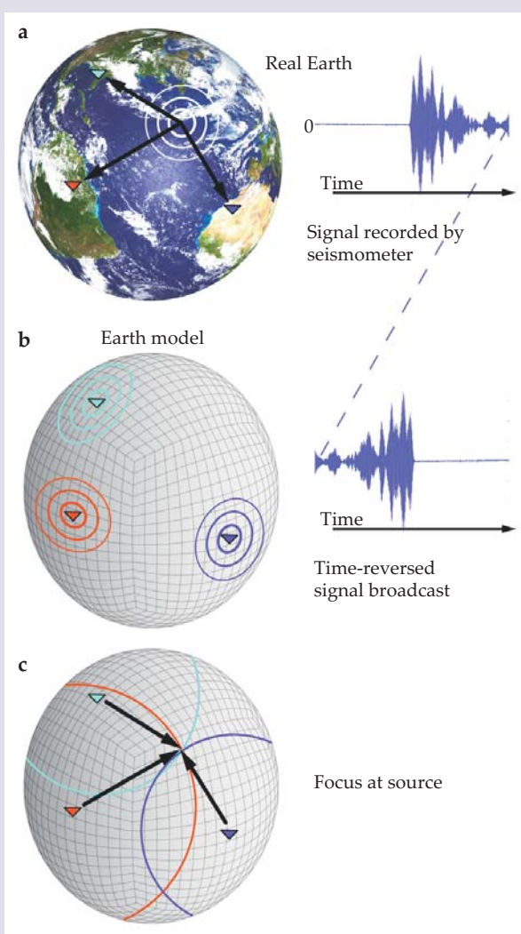
Figure 3. Time-reversal seismology. (a) A seismic signal radiating from its source is recorded by three distant stations. (b) The signals are time-reversed and, in a computer simulation, rebroadcast from their respective stations into a model Earth. (c) The time-reversed signals propagating through the model Earth converge at a focus, revealing the location and structure of the real source.
