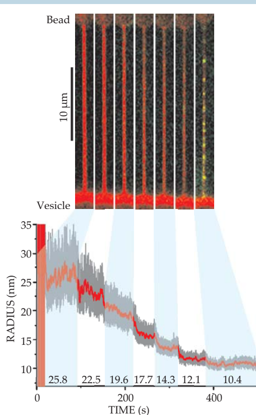
Figure 3. At low concentration dynamin molecules can't polymerize on a tube unless the tube's outside radius matches the molecules' inside radius. To obtain that result, Roux and his colleagues decreased the tube's radius in step-wise fashion giving dissolved dynamin molecules the opportunity to polymerize. As the sequence of micrographs shows, the fluorescently tagged dynamin (green) sticks to the tube only when its radius has reached 10.4 nm. The green dots represent nucleating spiral segments, not individual molecules, which are too small for the microscope to resolve. (Adapted from ref. 1.)
