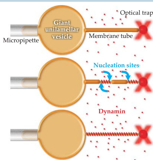
Figure 2. Dynamin's polymerization can be studied by fluorescently tagging dynamin molecules and watching to see whether they polymerize on the surface of a thin membrane tube. The tube is drawn from a giant unilamellar vesicle by affixing a bead to the GUV's membrane and tugging on it with an optical trap. The tube's radius is set by adjusting the negative pressure on the GUV through a micropipette. Measuring the force on the trapped bead yields the value of the radius. (Adapted from ref. 1.)
