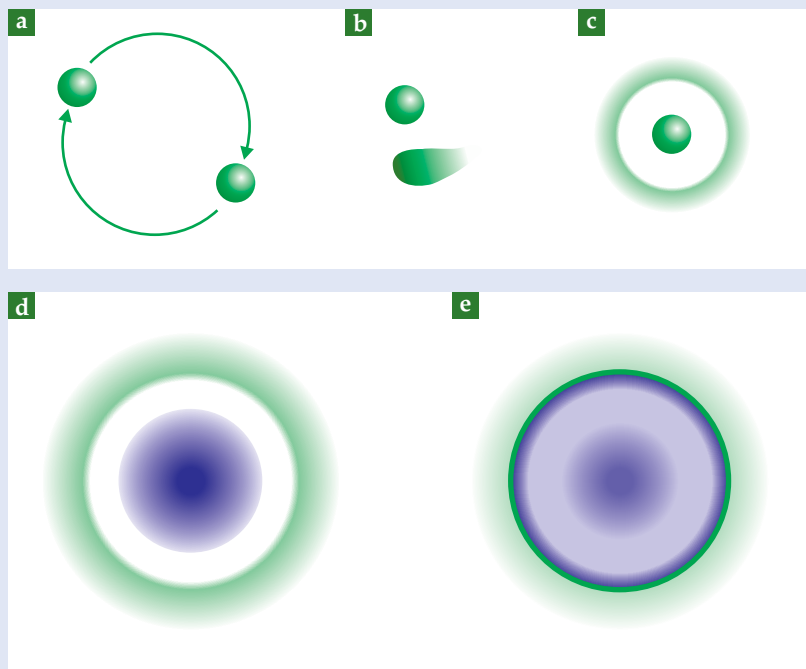
Figure 2. A supernova from two merging white dwarfs shown schematically. Carbon and oxygen are shown in green; fusion products are shown in purple. (a) White dwarfs orbit each other in a binary system. (b) The more massive dwarf tidally disrupts the less massive one. (c) Some of the disrupted white dwarf's mass forms a diffuse disk or envelope. (d) The central dwarf explodes, but the envelope remains intact. (e) Ejecta from the explosion collide with the envelope, initiating a shock wave that slows down the ejecta.
