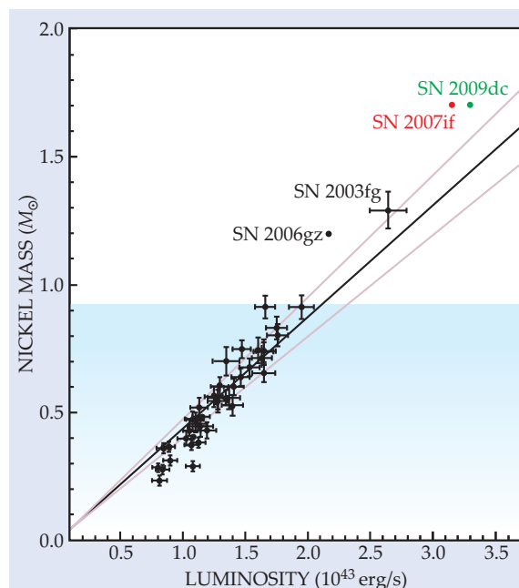
Figure 1. Overluminous supernovae SN 2003fg, SN 2006gz, SN 2007if, and SN 2009dc, compared with other type Ia supernovae from the Supernova Legacy Survey. The shaded blue region shows the range of nickel masses that can be produced by a Chandrasekhar-mass ( 1.4 M_{\odot} ) white dwarf. Although error bars are not shown for the newer data points, intervening dust is a source of significant uncertainty. The luminosities shown for SN 2006gz and SN 2009dc both assume that much of the emitted light was absorbed by dust; the value for SN 2007if assumes no dust absorption. (Adapted from ref. 1.)
