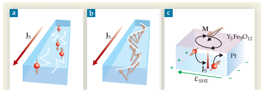
Figure 1. Spin currents in solids. Spin angular momentum J_s can be carried by (a) electron diffusion or by (b) spin waves, the collective precession of magnetic moments. (c) At the interface of an insulator such as yttrium iron garnet and a metal film such as platinum, angular momentum from the precession of the insulator's magnetization M can be pumped into the metal, where it appears as a conduction-electron spin current. By the inverse spin Hall effect, spin-orbit coupling deflects electrons of opposite spins in the same direction, whereby they accumulate on the same Pt edge. The charge imbalance sets up an electromotive force, E_{SHE} , measurable as a voltage. (Adapted from ref. 2.)
