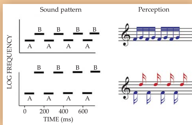
Figure 4. Perceptual segregation of tone sequences is studied by presenting listeners with a sequence of tones that alternate between two frequencies, A and B. When the frequency difference between them is small (top row), listeners perceive a single coherent stream of tones. But when it is large (bottom row), the sequence breaks apart perceptually into two unrelated streams, indicated by the colors.
