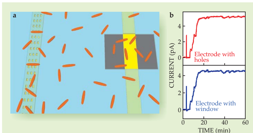
Figure 1. Evidence for indirect, shuttle-mediated electron transfer. (a) The microbial fuel cell fashioned by Charles Lieber, Bradley Ringeisen, and colleagues featured two types of nanoelectrodes: One, shown at left, was exposed via nanoholes small enough to preclude contact with microbes; the other, shown at right, had large window exposures that allowed the microbes direct access. (b) Both types of electrodes generated nearly identical current, and that current vanished when shuttle molecules were flushed from the system, all of which suggests an indirect mechanism for electron transfer. (Adapted from ref. 1.)
