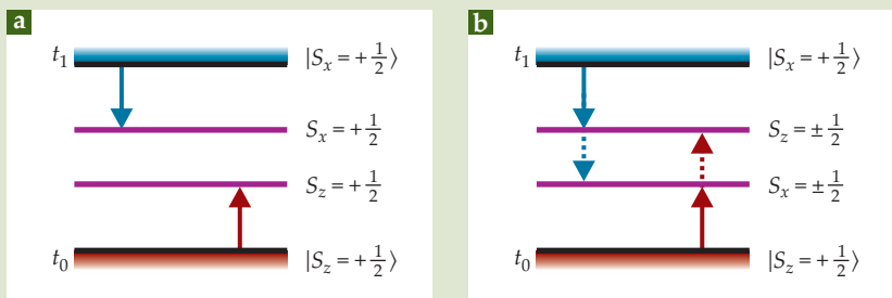
Figure 2. Measuring both the x and z spin components of a spin- \frac{1}{2} particle in the interval between the pre- and postselections of figure 1 yields different results depending on the time order of the two measurements. (a) If the first interim measurement is along the direction of the preselection and the second interim measurement is along the postselection direction, both measurements are determined by the selections. (b) Reversing the order of the interim measurements destroys that certainty.
