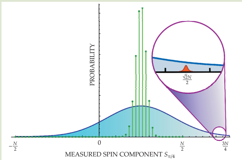
Figure 3. Probability distributions for different outcomes of the measurement of the spin component S_{\pi/4} of a system of N spin- \frac{1}{2} particles preselected in the state |S_z = +N/2\rangle . The green histogram represents measurement outcomes for an ideal measurement without postselection. The blue curve represents the probabilities in an approximate measurement. After postselection for the very improbable state |S_x = +N/2\rangle , only the red distribution way out in the tail survives.
