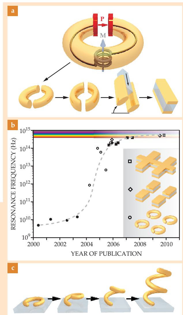
Figure 1. (a) A split-ring resonator (SRR) is essentially a miniature inductive-capacitive circuit. If many such circuits are packed together, they effectively become a material with a polarization \mathbf{P} and magnetization \mathbf{M} . A sequence of continuous deformations, connected by arrows, turns the SRR into a cut-wire pair separated by a dielectric (gray). Such resonators form the basis for artificial magnetism at optical frequencies. (b) The dramatic increase in resonance frequency in magnetic (open symbols) and negative-refractive-index (filled symbols) metamaterials achieved by several research groups over a few short years started to level off in 2006 due to a metal’s finite plasma frequency, which imposes a fundamental limit on the resonance frequency. 7,8 (c) A three-dimensional metal helix can be formed by pulling one end of an SRR out of the plane. In the metal helix, \mathbf{M} can point parallel to the electric field and lead to giant optical activity and circular dichroism.
