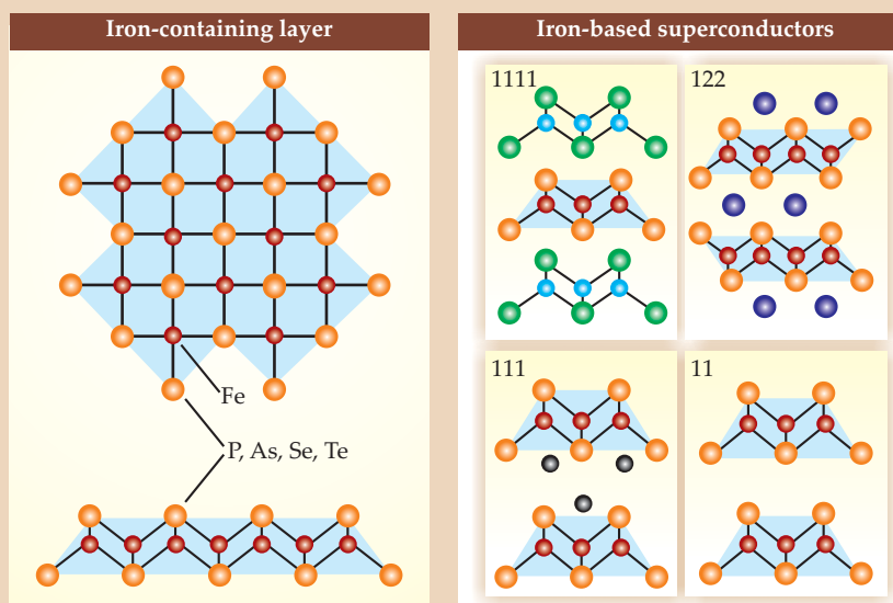
Figure 1. Superconductivity in the new Fe-based materials takes place in a corrugated layer made up of Fe and one of two pnictogens (phosphorus, arsenic) or one of two chalcogens (selenium, tellurium). Four structural families, depicted schematically on the right, incorporate the layer with a characteristically different interlayer. In the 1111 family, the interlayer consists of a rare earth (blue) and oxygen (green); in the 122 family, an alkaline earth (violet); and in the 111 family, an alkali (gray). There's no interlayer in the 11 family; to preserve the layer's charge balance, the pnictogen is replaced by a chalcogen. (Adapted from K. Ishida, Y. Nakai, H. Hosono, J. Phys. Soc. Jpn. 78 , 062001, 2009.)
