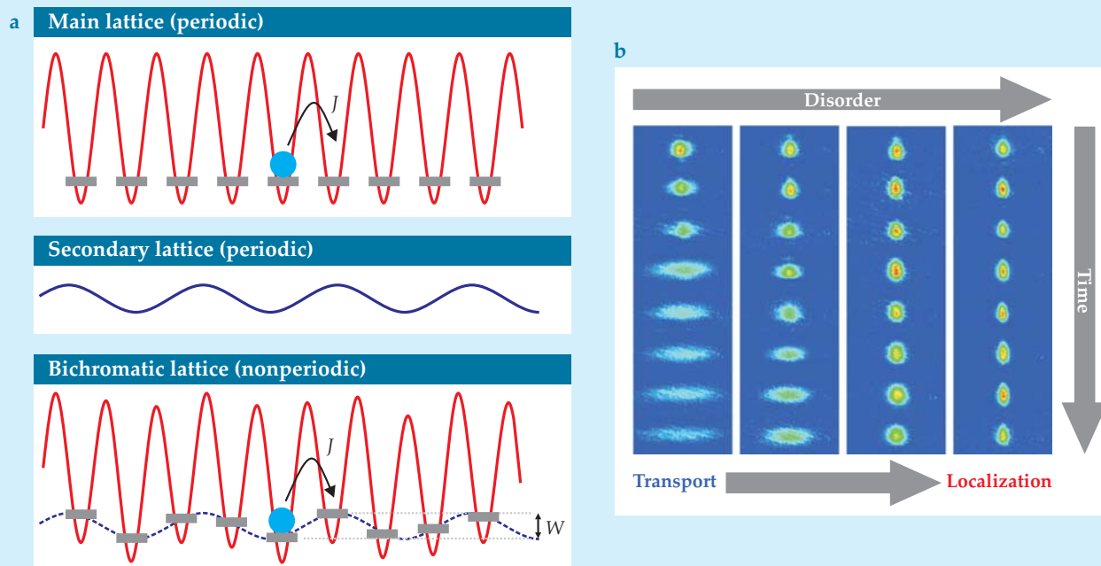
Figure 4. A bichromatic lattice simulates solid-state model. Loaded in a laser standing wave, an ultracold atom (blue) experiences a periodic potential. (a) The tunneling energy J can be controlled by changing the intensity of the main standing wave. A second, weaker optical lattice with an incommensurate spacing breaks the translational invariance and scrambles the site energies, as in the original solid-state model introduced by Philip Anderson. (b) Time-resolved images of almost noninteracting potassium-39 atoms. The atoms are first loaded into a few central sites of the bichromatic lattice and then observed diffusing into that nonperiodic structure. An increase in disorder leads to a decrease in diffusion and eventually its absence when the amount of disorder W becomes on the order of J .
