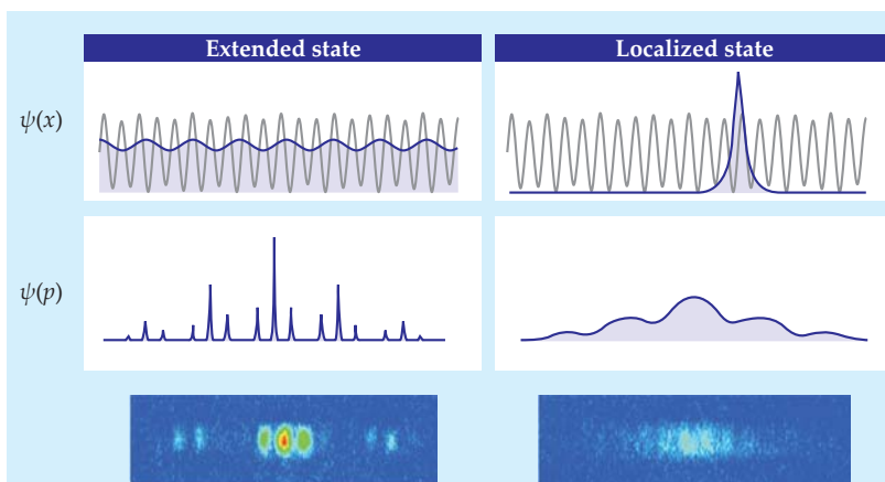
Figure 5. Imaging the phase transition in momentum space. When the atomic wavefunction is extended all over the bichromatic lattice, narrow peaks are recorded in the momentum distribution. When the atomic wavefunction is localized, a broad momentum spread is observed, as expected from the uncertainty principle. The false-color images in the bottom row are experimental maps of the momentum distribution recorded after a time-of-flight expansion in free space.
