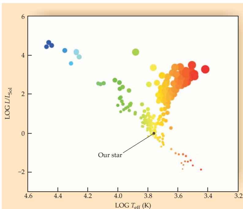
Figure 1. The Hertzsprung–Russell diagram, a plot of luminosity L (relative to the Sun's luminosity L_{\text{Sol}} ) against temperature T_{\text{eff}} , has been used by astronomers for nearly a century to help categorize stars and to track their life cycles. In this HR diagram of more than 250 stars whose sizes have been measured by interferometry, the circles' sizes are proportional to the logarithms of the stars' radii, and color is a reflection of the photospheric temperature shown on the horizontal axis. Prior to the availability of interferometric measurements, some qualitative conclusions could be drawn about stars' sizes based on their positions on the plot: Cooler, faint stars at the bottom right are expected to be small, and more luminous cool stars at the top right must be giants. That understanding is now becoming quantitative with the direct diameter measurements provided by interferometry. The diagonal line from top left to bottom right is the main sequence, where stars spend the most stable, and frequently most lengthy, part of their lives. Our star, the Sun, is a main-sequence star. (Courtesy of Tabetta Boyajian, Georgia State University.)
