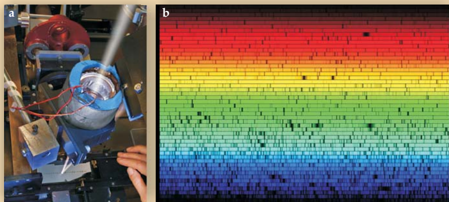
Figure 2. Doppler spectroscopy
