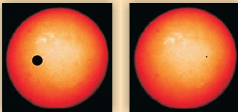
Figure 4. The transit of an exoplanet across the disk of its parent star is simulated by an image of the Sun and dark spots representing (left) a Jupiter-size and (right) an Earth-size planet. A transiting Jupiter would block about 1% of a Sun-like star's light. An Earth's dimming signal would be 100 times weaker. (Courtesy of NASA.)
