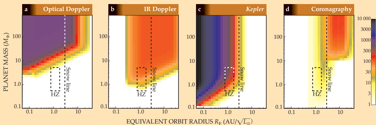
Figure 5. Depth-of-search plots compare the discovery potential of planet-search surveys of different sizes and techniques. Plotted are the distributions of a figure-of-merit function S(M, R_E) over the masses M and thermal-equivalent orbital radii R_E (defined in the text) of exoplanets being looked for. At each point in the M, R_E plane, S is the sum, over all the survey's stars, of the probabilities of detecting such a planet if it were indeed orbiting that particular star. The dashed rectangle marks the habitable zone (HZ) of radii that allow liquid water and masses suitable for both substantial atmospheres and rocky surfaces. Beyond the marked snow line, icy material in the early stellar system was available for rapid formation of planetary cores. (a) A large-scale Doppler survey covering 1000 stars over 15 years at optical wavelengths. (b) A smaller Doppler survey covering 120 cool, low-mass stars over 5 years at IR wavelengths. (c) The recently launched Kepler mission searching for transiting exoplanets. Kepler can only detect a planet passing directly between it and the face of the host star. Therefore the detection probability drops from about 10% for orbits close to the star to much less than 0.1% for large orbits. Kepler will survey about 100 000 stars, so S drops from 10 000 to less than 100 with increasing orbital radius. (d) A proposed direct-imaging survey using an orbiting 2.5-m telescope operating with an advanced coronagraph and spectroscopic capability. The telescope's aperture would limit the mission's range to a few hundred nearby stars.
