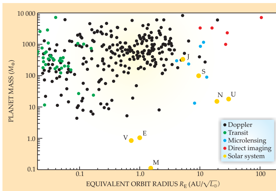
Figure 1. For more than 300 planets already discovered, mass (in units of Earth's mass M_{\oplus} ) is plotted against R_E , a thermal-equivalent orbital radius given by R/\sqrt{L} , where R is the actual radius (in astronomical units) and L is the parent star's luminosity (in units of the Sun's luminosity L_{\odot} ). So planets with the same R_E around very different stars experience the same intensity of stellar irradiation, and planets orbiting in the so-called habitable zone of Earth-like temperatures all have R_E near 1. Planets of our solar system are labeled by their initials. The exoplanets are colored according to the technique by which each was first detected.
