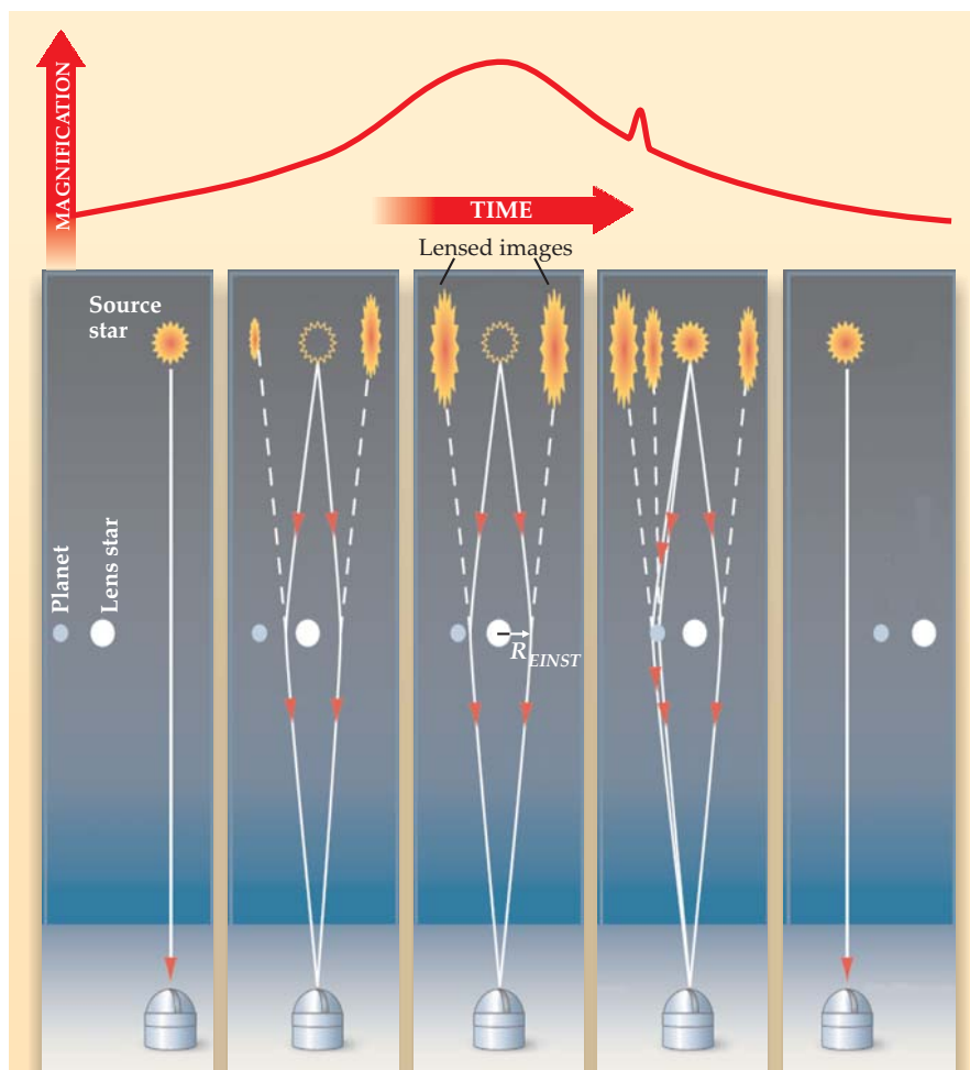
Figure 3. Microlensing can reveal exoplanets. By gravitational bending of light, a foreground lensing star passing near the sightline to a much brighter background source star displaces, distorts, and often duplicates the latter's image. If the Einstein radius R_{\text{Einst}} , the characteristic size parameter of the lensing event, subtends an angle too small for a telescope to resolve, the observer does not see multiple images of the source star but only an ephemeral brightening of its light curve (red curve, top) as the lens star passes by. A planet accompanying the lens star at a distance comparable to R_{\text{Einst}} can reveal itself as a bump on the light curve. (Adapted from David Bennett's website: http://www.nd.edu/~bennett/moa53-ogle235 .)
