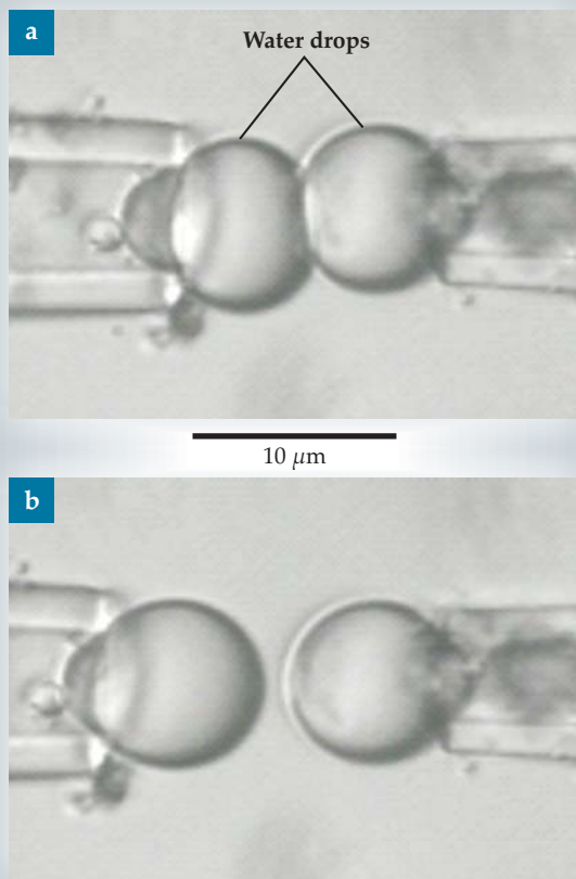
Figure 6. Droplets of water in diluted bitumen are coated with a skin of submicron particles. As a result, when they are (a) forced into contact and (b) allowed to separate, no coalescence takes place. (Courtesy of Anthony Yeung, University of Alberta.)
