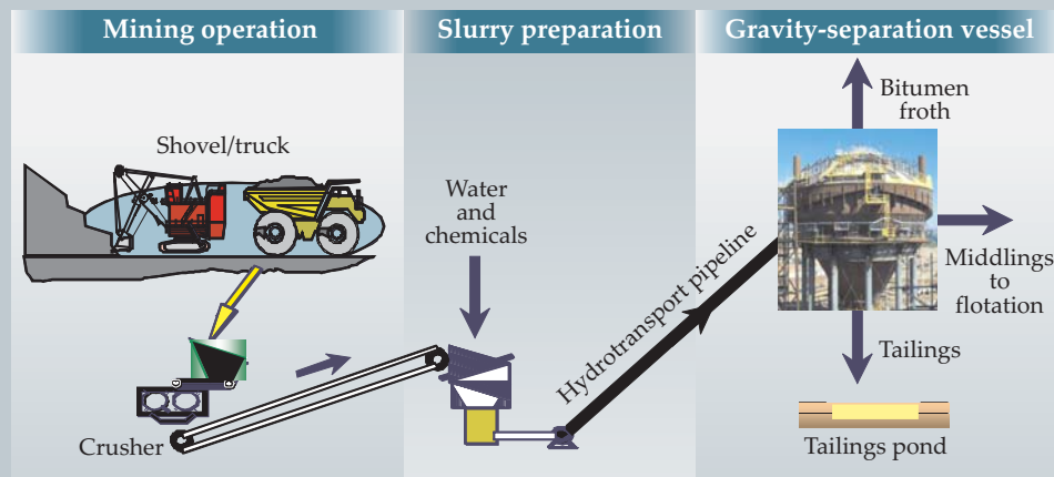
Figure 2. Bitumen production
