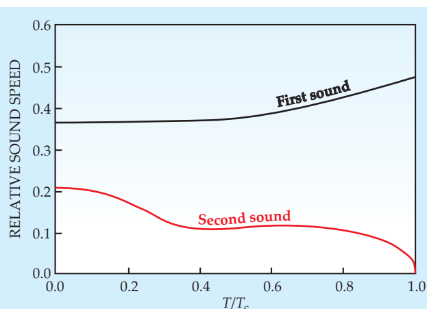
Figure 5. Calculated first- and second-sound velocities in a uniform superfluid gas of ultracold Fermi atoms at unitarity, the point at which the atomic scattering length is infinite. The velocities are given relative to the Fermi velocity, and the temperature T is scaled to the superfluid transition temperature T_c . (Adapted from ref. 13.)
