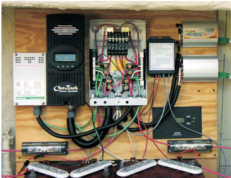
Figure 3. Power center for my dual PV system. Only half the parts are necessary for a more typical single system. Cut off at the bottom edge of the photo are two 12-V, 150-Ah batteries (one for each system), and immediately above them are 110-A class-T fuses. At left are two charge controllers. The black one is a maximum power-point tracking charge controller, as described in the text; it is certainly overkill for this small system. In the upper right are two 400-W inverters. Below them is an MPPT charge controller not currently used. To the left of the inverters is the monitoring system, capable of measuring two voltages and three currents. In the center is the exposed breaker box, showing three breakers per system, four shunts for current measurement (I use only three
