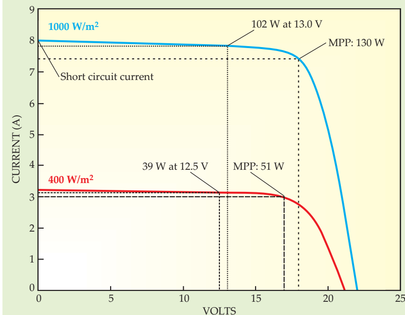
Figure 4. Current-voltage curves for a photovoltaic panel rated at 130 W at 25 °C. The blue curve shows full illumination; the red curve shows 40% illumination. Typical PV panels, with 36 cells in series, have an open-circuit voltage of around 22 V. Maximum power is typically delivered at around 15–18 V. At lower voltages, the PV current saturates; in full sun the saturation current is called the short-circuit current. The maximum power point (MPP) is indicated for both curves, as is the reduced power achieved by extracting current at typical battery voltages.
