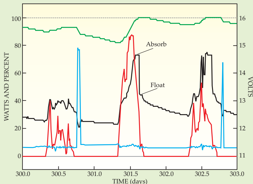
Figure 5. Sample data for a 130-W solar panel powering an entertainment system. Day 300 had a heavy but variable overcast; day 301 was mostly sunny; day 302 was cloudy. The red curve traces the solar power delivered by the panel to the charge controller, and the blue curve traces the load. Note the constant “off” load plus brief intervals of television usage. The black curve is battery voltage, as indicated on the right-hand scale. The battery reached absorption stage on days 301 and 302 and also showed intervals of float stage—indicating a fully charged battery—at the end of both days. The green curve indicates battery charge as a percent of capacity. The first day made only a small positive contribution to the battery charge, but the sunny day that followed made up for the deficit. Note that the falling edge of the solar
