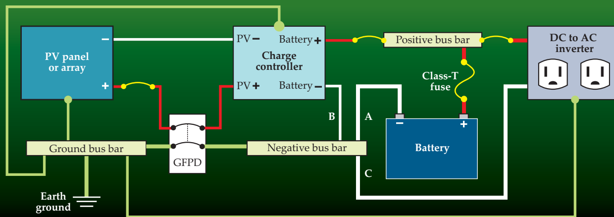
Figure 2. Circuit diagram for a standalone photovoltaic system. The breakers (yellow arcs) serve as overcurrent protection and disconnect simultaneously, but they can be implemented as fuses and disconnect switches. If the PV panels are not attached to a dwelling, the ground-fault protection device (GFPD) can be eliminated and the same bus bar, a metal strip that allows branch connections, can be used for negative and ground. All modules have grounded frames. In-line shunts can be placed at locations A, B, and C for measuring net battery current, solar input current, and load current, respectively—although, since those currents obey a sum rule, any two will suffice. Ground wires are green, negative white, and positive red.
