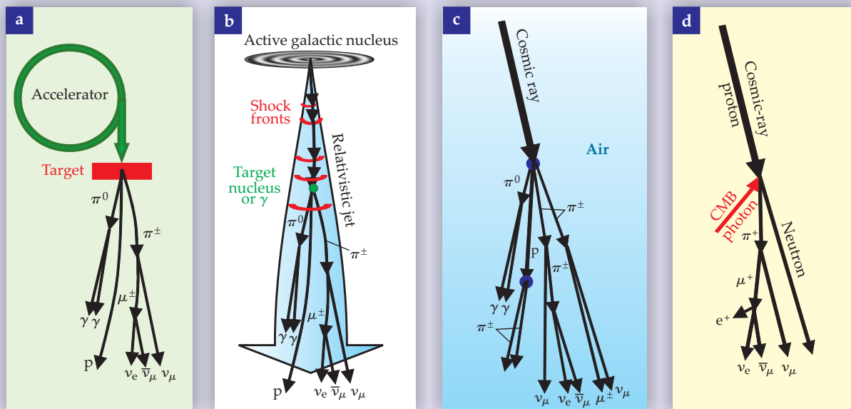
Figure 2. Four neutrino sources. (a) An accelerator proton beam collides with nuclei in a target to produce mesons. Their decay products include neutrinos of various flavors (see box 1). (b) Shock fronts in a relativistic jet emerging from an active galactic nucleus or other high-energy astrophysical source accelerate nuclei that then create mesons when they hit surrounding radiation or gas. (c) An air shower initiated by a cosmic-ray nucleus hitting Earth's atmosphere produces mesons and their decay products. (d) A cosmic-ray proton with energy above the Greisen-Zatsepin-Kuzmin threshold can produce a \pi^+ simply by colliding with a cosmic-microwave-background photon. A resulting decay neutrino can have energy as high as 10^{20} eV.
