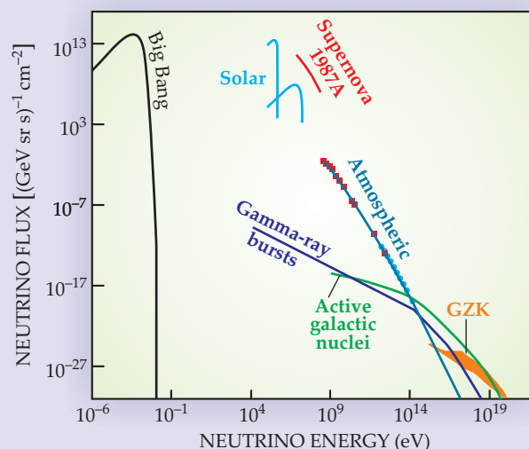
Figure 1. The cosmic neutrino spectrum. A low-energy background left over from the Big Bang is believed to suffuse the cosmos. Neutrinos from the Sun confirmed the fusion processes that provided its heat, and they yielded the first evidence of neutrino flavor oscillation. Neutrinos have also been detected from the nearby supernova explosion 1987A. Much of the spectrum of atmospheric neutrinos from cosmic-ray air showers has been measured by the Fréjus underground detector (orange data points) in France and the AMANDA detector (blue dots) deeply embedded in ice near the South Pole. Not yet observed are neutrinos expected from cosmological point sources such as gamma-ray bursts and active galactic nuclei. The most energetic neutrinos are expected from the decay of pions created in collisions between cosmic-microwave-background photons and cosmic-ray protons with energies above 4 \times 10^{19} eV (the Greisen-Zatsepin-Kuzmin threshold).
